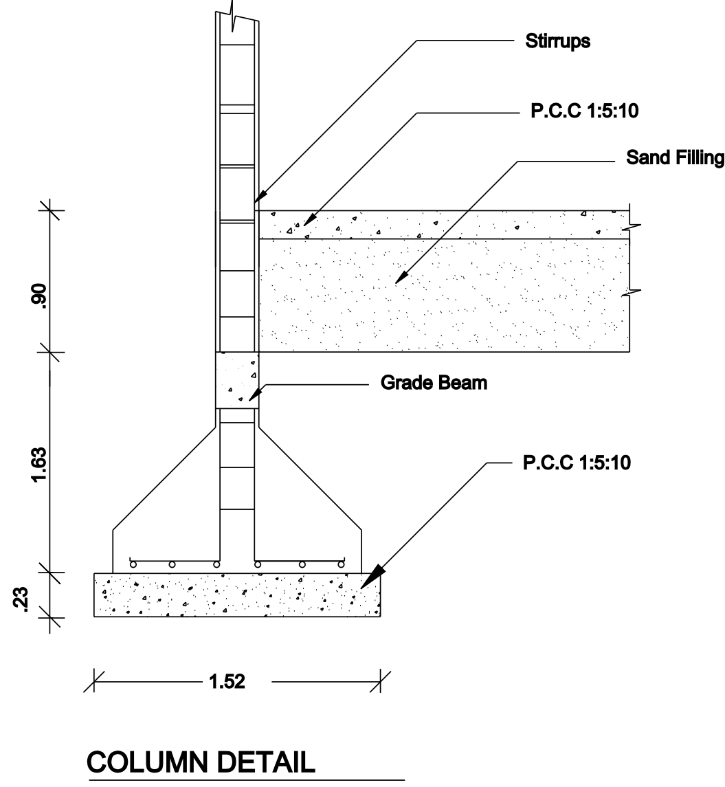
COLUMN DETAIL
