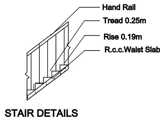
STAIR DETAILS
