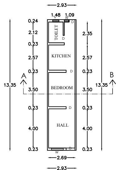
PRO GROUND FLOOR PLAN
