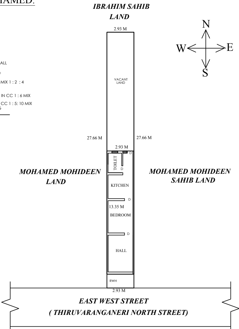
SITE PLAN
