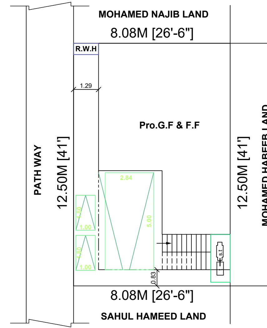
SITE PLAN (NOT FOR SCALE)
