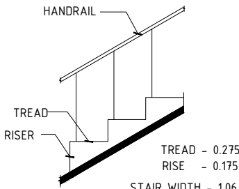
STAIRCASE DETAILS NTS
