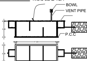
SEPTIC TANK AND TRENCH NTS
