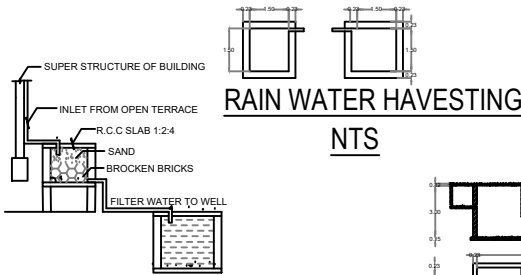
DETAILS OF FILTER BED & WELL NTS
