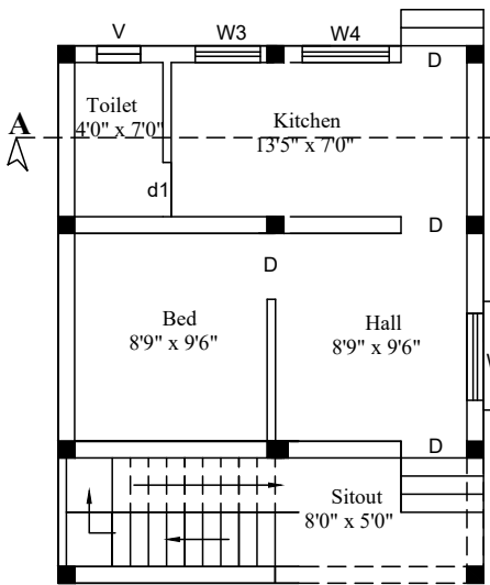
EXTG. GROUND FLOOR PLAN
