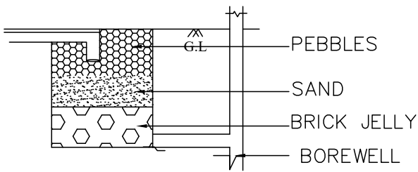
RAINWATER FILTRATION
