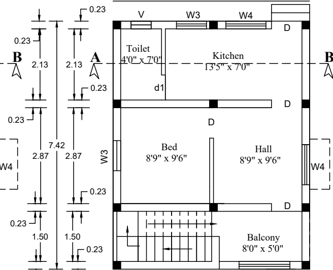
PRO. FIRST FLOOR PLAN
