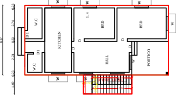
GROUND FLOOR PLAN (EXISTING)
