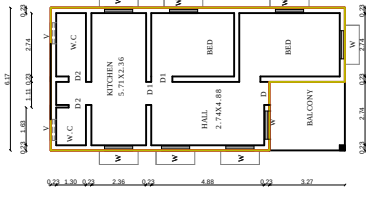
FIRST FLOOR PLAN (PROPOSED)
