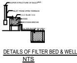
DETAILS OF FILTER BED & WELL
