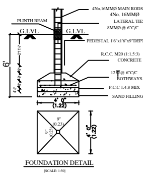
FOUNDATION DETAIL
