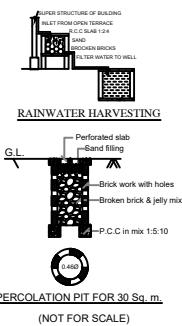
PERCOLATION PIT FOR 30 Sq. m.
