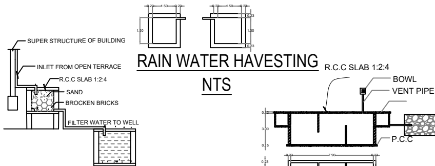
DETAILS OF FILTER BED & WELL NTS
