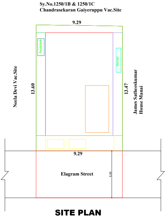
SITE PLAN
