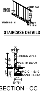
SECTION - CC
