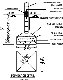
FOUNDATION DETAIL
