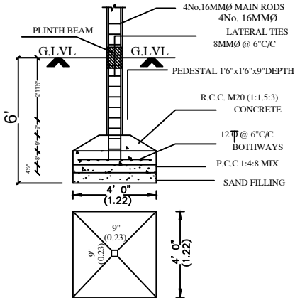
FOUNDATION DETAIL (SCALE: 1:50)
