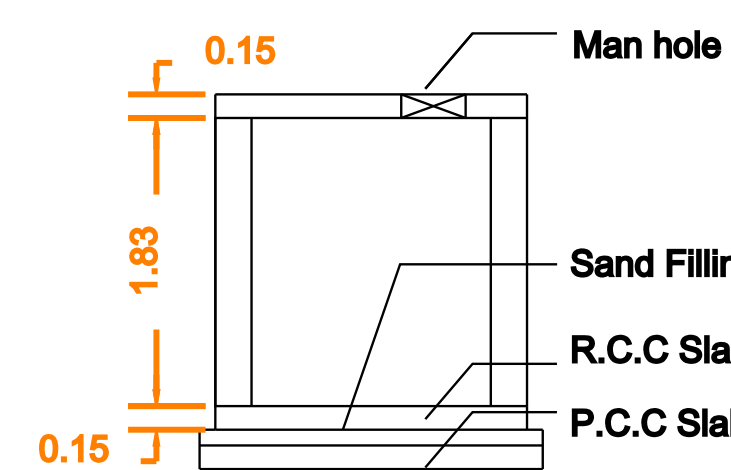
SUMP DETAILS
