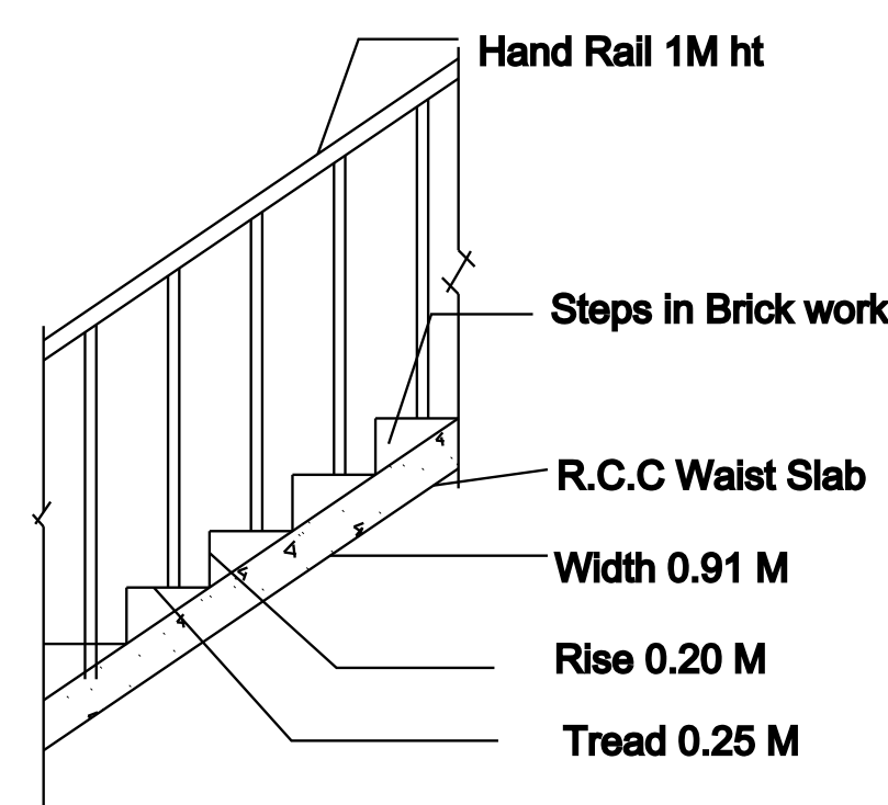
STAIRCASE DETAILS
