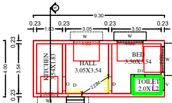
PRO. GROUND FLOOR PLAN
