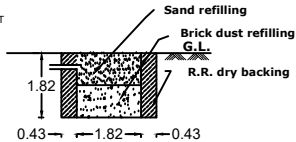
DETAILS OF RAIN WATER HARVESTING Dwg:1A
