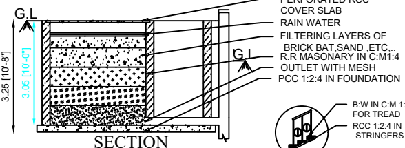
RAIN WATER HARVESTING OF RECHARGE TRENCH METHOD
