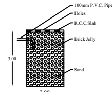
SECTION OF RAIN WATER COLLECTING TANK
