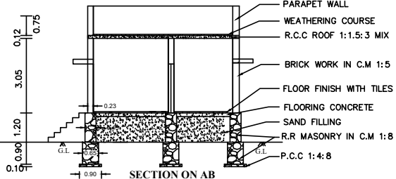
SECTION ON AB Mr. Thangapandi House 42'0" (12.80 m)
