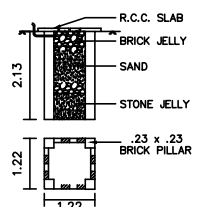
PLAN & SECTION OF RAIN WATER COLLECTION WELL
