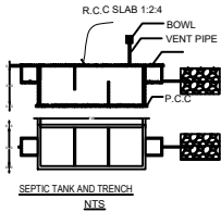
SEPTIC TANK AND TRENCH NTS
