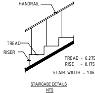
STAIRCASE DETAILS NTS
