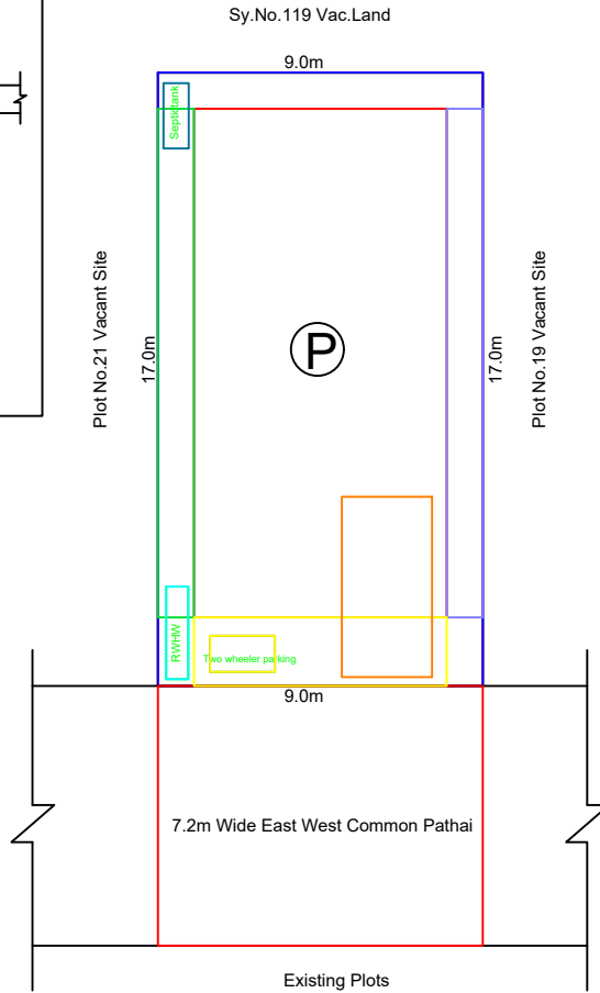
SITE PLAN
