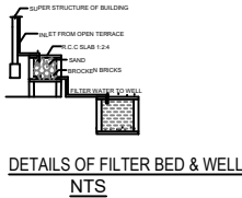
RAIN WATER HARVESTING NTS
