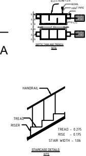
STAIRCASE DETAILS NTS
