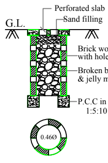
PERCOLATION PIT (NOT FOR SCALE)
