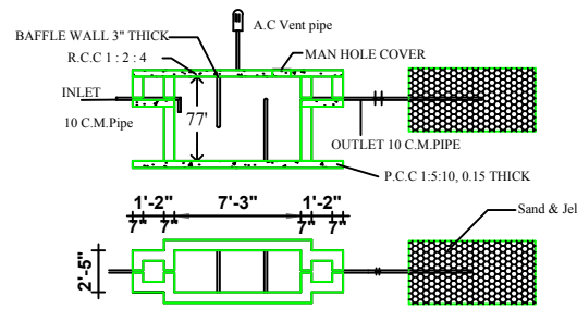
Septic tank and trench
