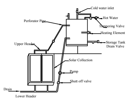
Details Of Solar Water Heater (NTS)
