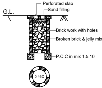
PERCOLATION PIT FOR 30 Sq. m.
