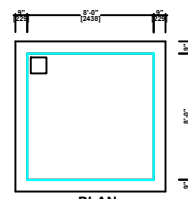
DETAILS OF COLLECTION SUMP FOR RAIN WATER HARVESTING OF ROOF TOP RAIN WATER RW_H_CAPACITY_L=5000LTRS
