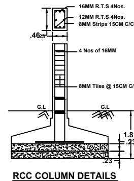
RCC COLUMN DETAILS
