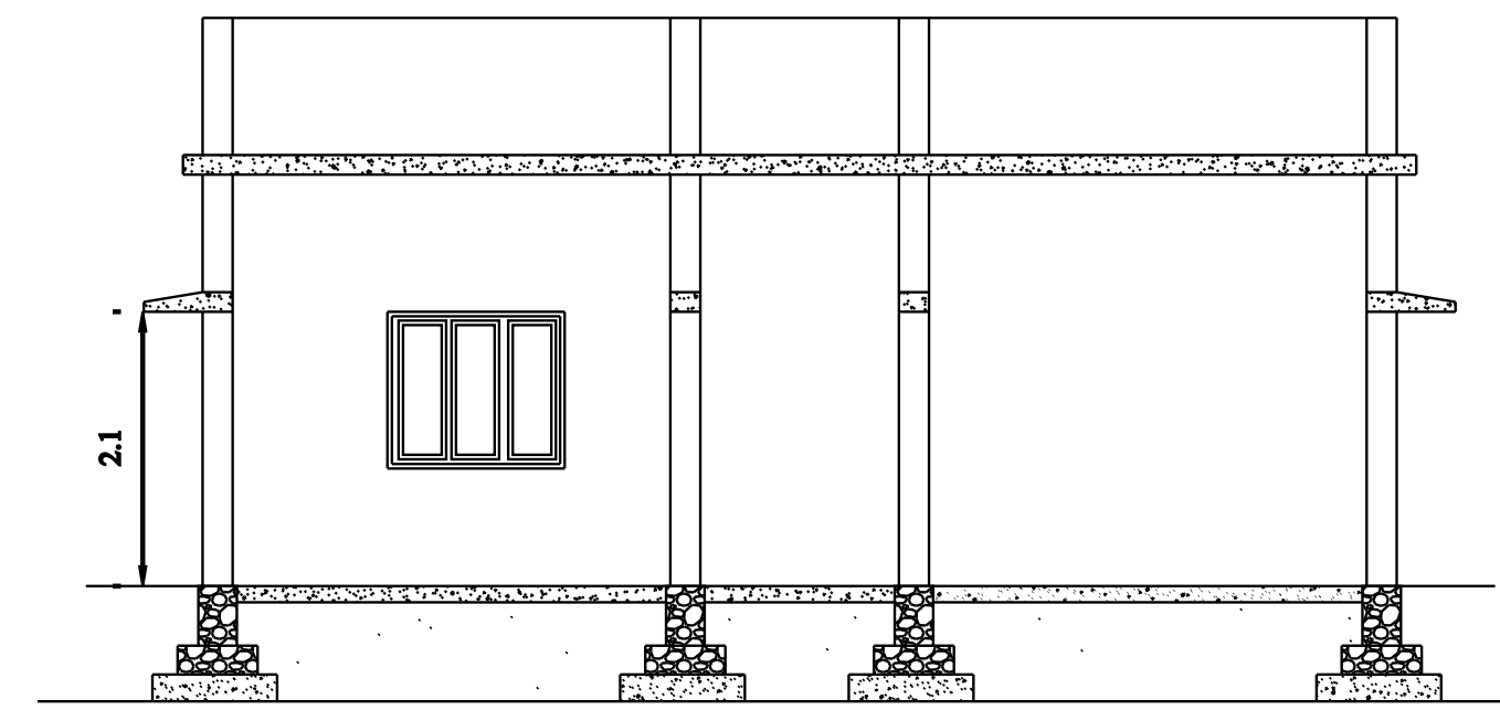
SECTION
