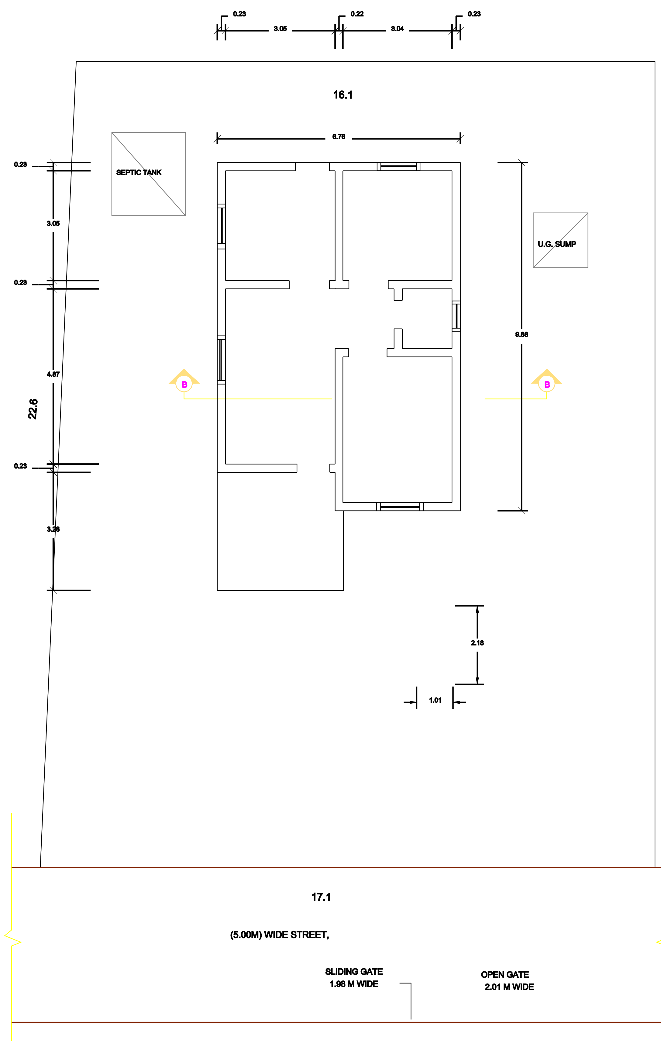
GROUND FLOOR
