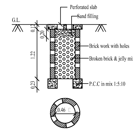
PERCOLATION PIT FOR 30 Sq. m. (Scale:- 1:50)
