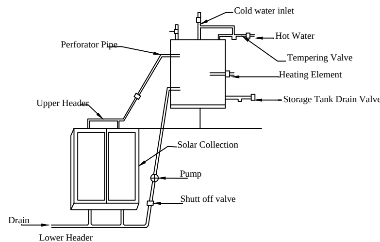
Details Of Solar Water Heater (NTS)
