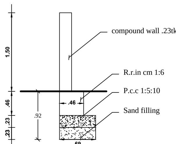
Compound Wall Detail
