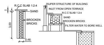
PERCOLATION PIT
