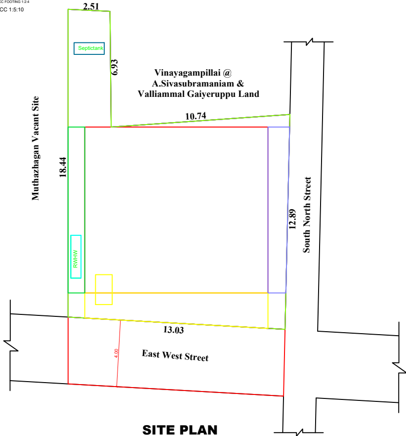
SITE PLAN
