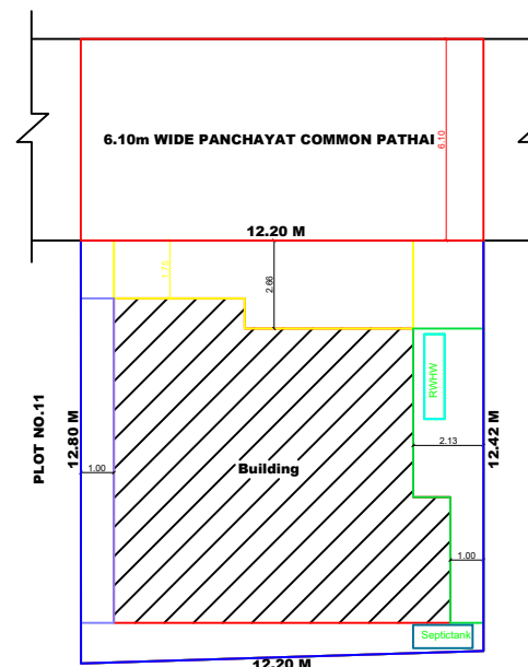
LOCATION PLAN
