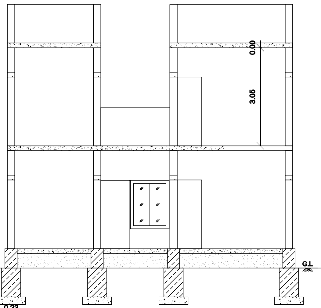
SECTION 'AA'
