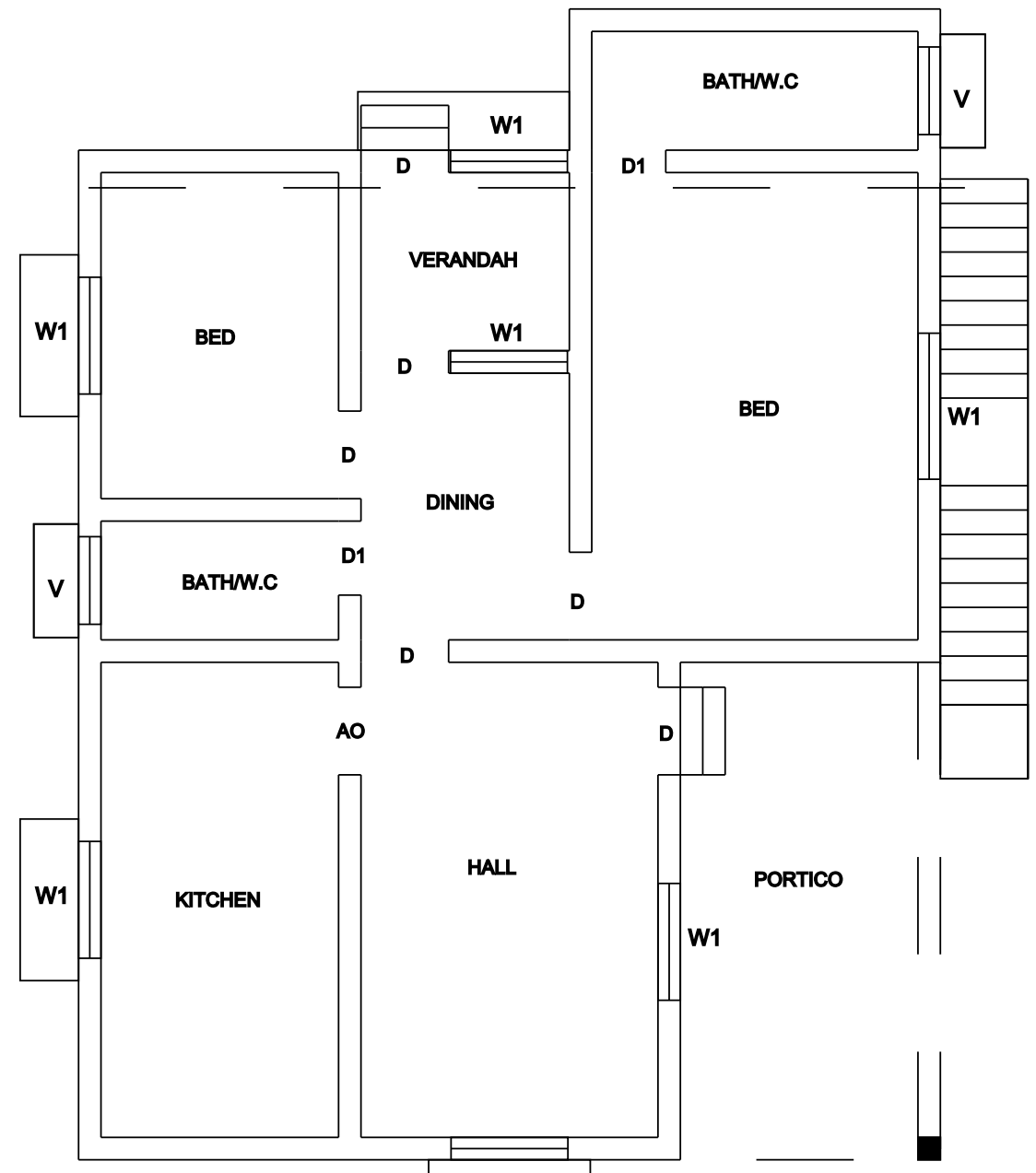
GROUND FLOOR
