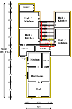
EXG.GROUND FLOOR PLAN
