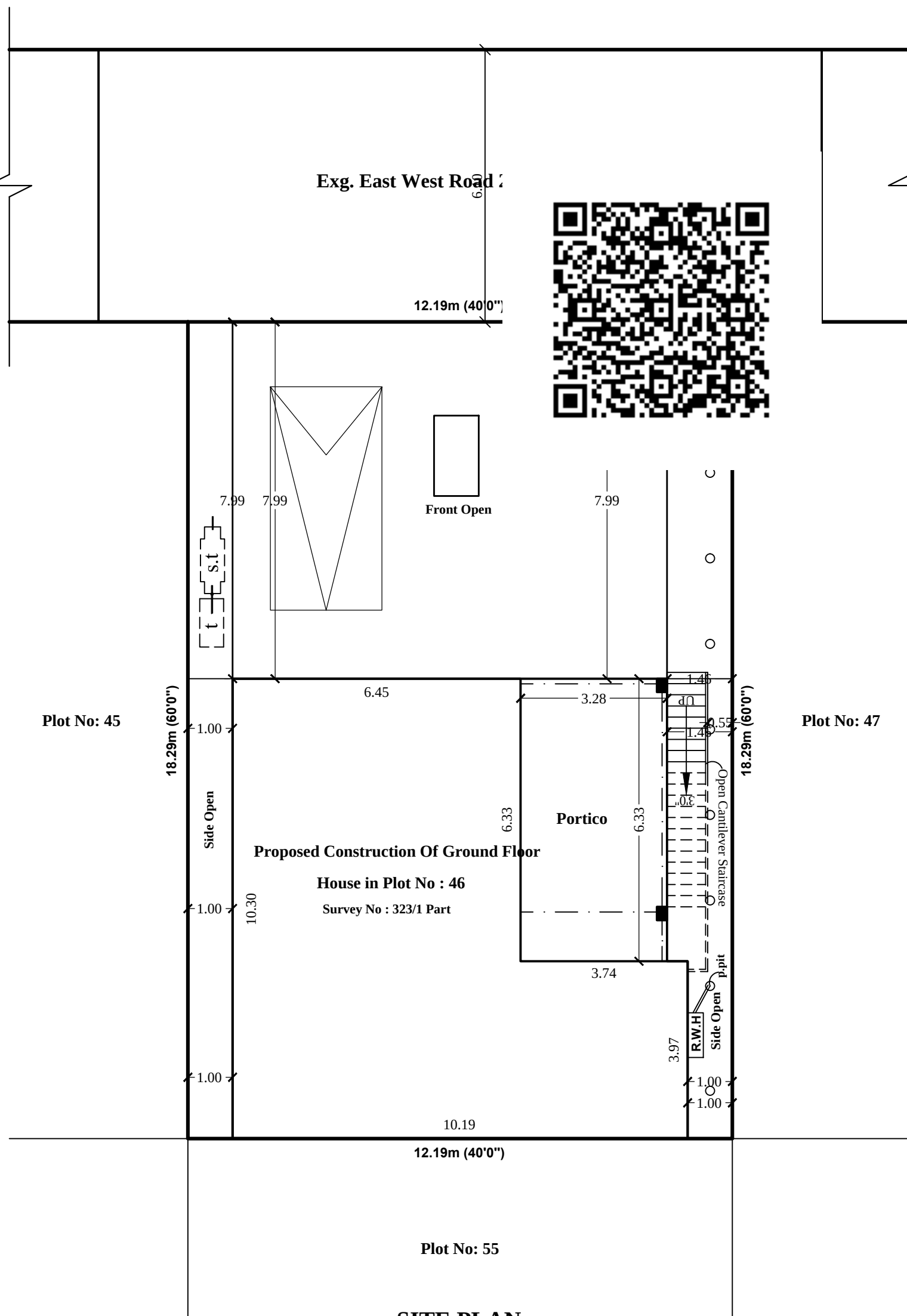
SITE PLAN
