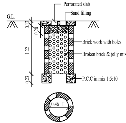
PERCOLATION PIT FOR 30 Sq. m. (Scale:- 1:50)
