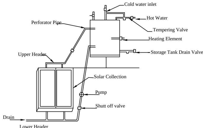
Details Of Solar Water Heater (NTS)
