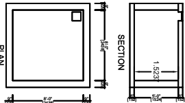
DETAILS OF COLLECTION SUMP FOR RAIN WATER HARVESTING OF ROOF TOP RAIN WATER RWH CAPACITY 1,50,000 LTRS
