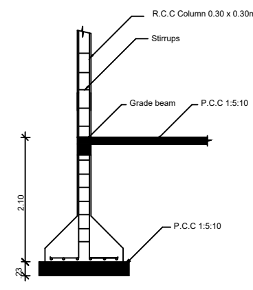
COLUMN DETAIL
