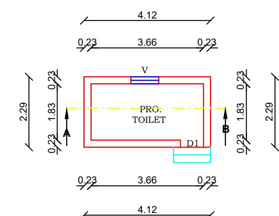
GROUND TOILET FLOOR
