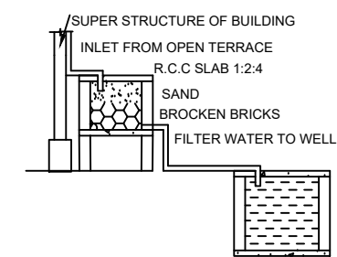
RAINWATER HARVESTING
