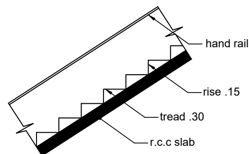
STAIR
