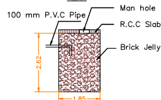
RAINWATER COLLECTION TANK
