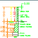
COMPOUND WALL DETAIL
