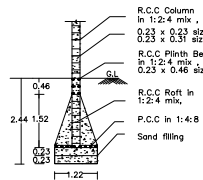
COLUMN DETAILS
