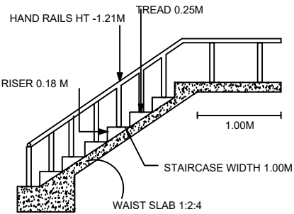
STAIRCASE DETAILS
