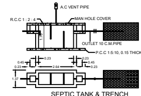
SEPTIC TANK & TRENCH
