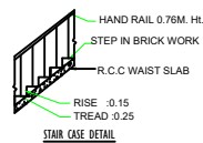
STAIR CASE DETAIL
