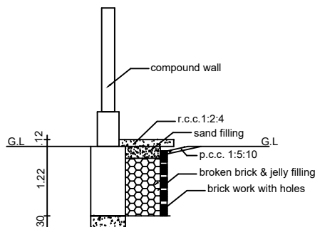
PLINTH BOUNDARY PERCOLATION PIT
