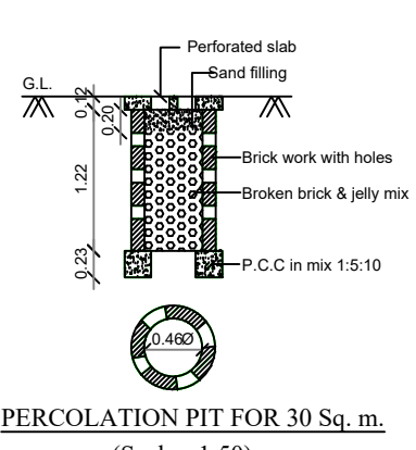
PERCOLATION PIT FOR 30 Sq. m. (Scale:- 1:50)
