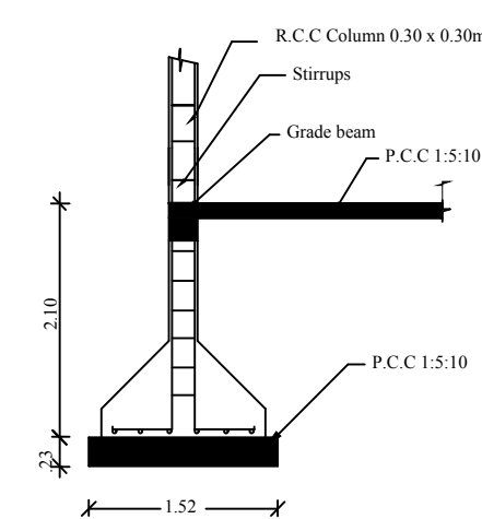
Column Detail
