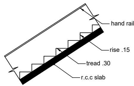
STAIR
