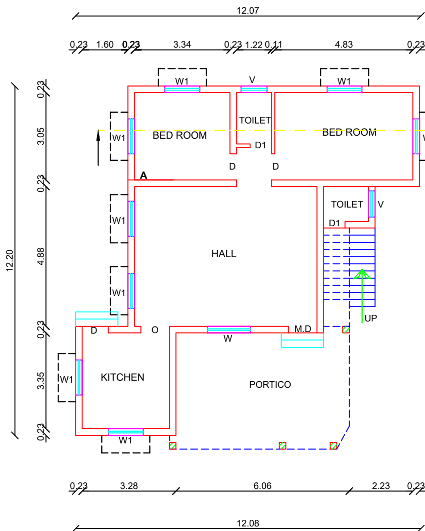
EXG. GROUND FLOOR PLAN
