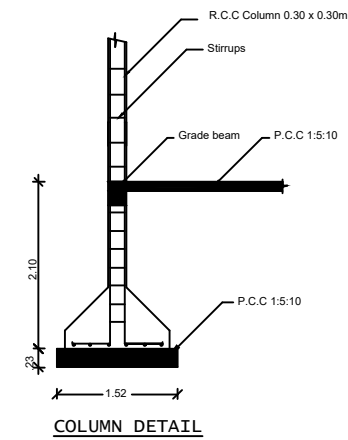
COLUMN DETAIL
