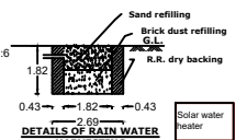
DETAILS OF RAIN WATER HARVESTING Dwg:1A
