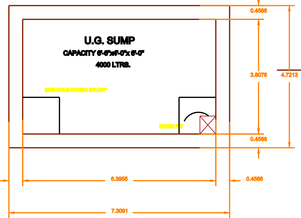
SUMP DETAIL
