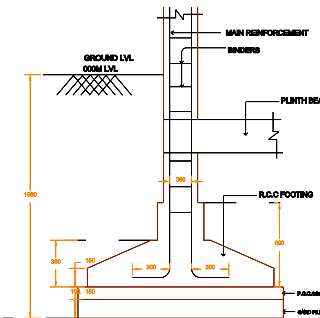
TYPICAL SECTION OF R.C.C COLUMN FOUNDATION SCALE: 1"=3'0"
