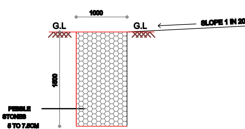
SECTION OF PEBBLE TRENCH
