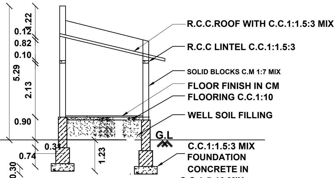
SECTION ON G1G2"
