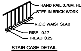
STAIR CASE DETAIL
