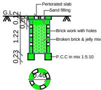
PERCOLATION PIT FOR 30 Sq. m. (Scale:- 1:50)
