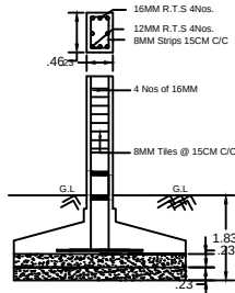
RCC COLUMN DETAILS
