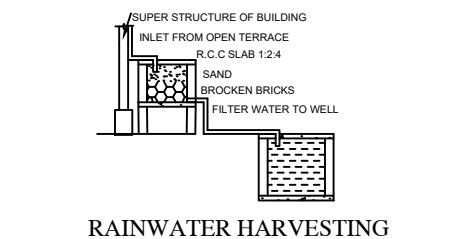
RAINWATER HARVESTING
