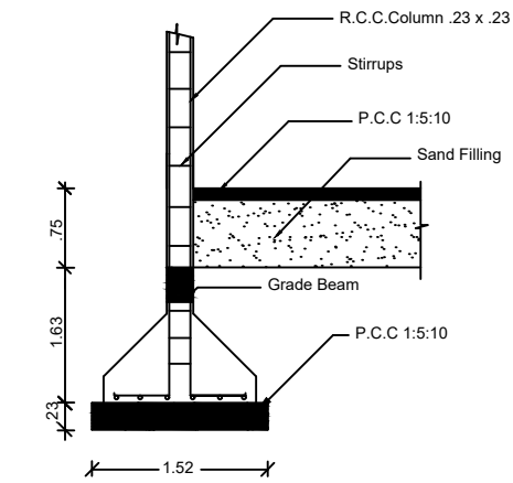
COLUMN DETAIL
