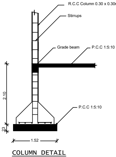
COLUMN DETAIL
