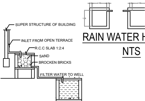
DETAILS OF FILTER BED & WELL NTS
