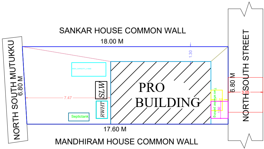
SITE PLAN
