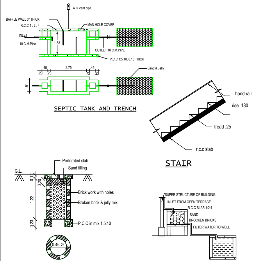
PERCOLATION PIT FOR 30 Sq.m. RAINWATER HARVESTING (Scale:- 1:50)
