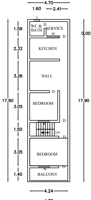
PRO FIRST FLOOR PLAN
