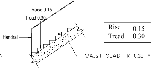
STAIRCASE DETAIL
