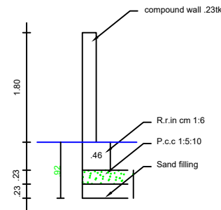
Compound wall Detail SCALE : (1:50)
