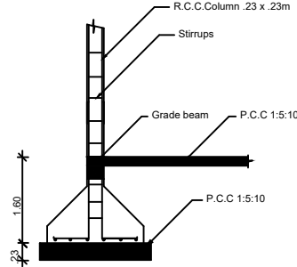
COLUMN DETAIL
