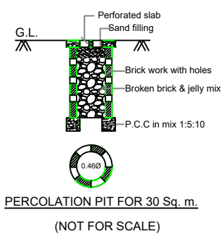
RAINWATER HARVESTING
