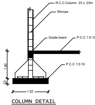
COLUMN DETAIL
